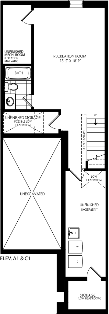
OPT. FINISHED LOWER LEVEL
