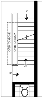
STAIR CONDITION FOR FINISHED LOWER LEVEL
