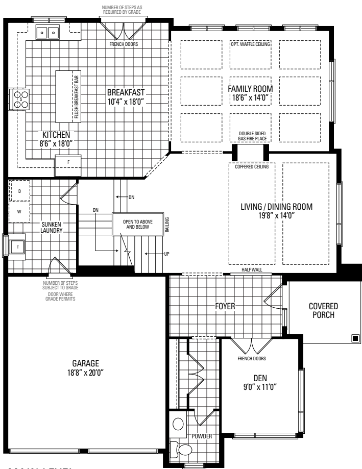
MAIN LEVEL
