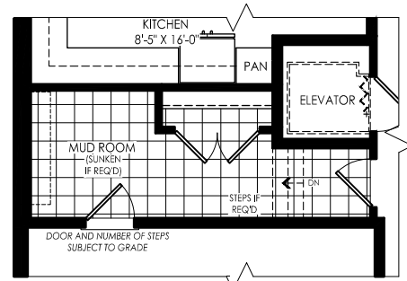
PARTIAL MAIN LEVEL FOR OPT. ELEVATOR
