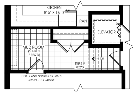
PARTIAL MAIN LEVEL FOR OPT. ELEVATOR
